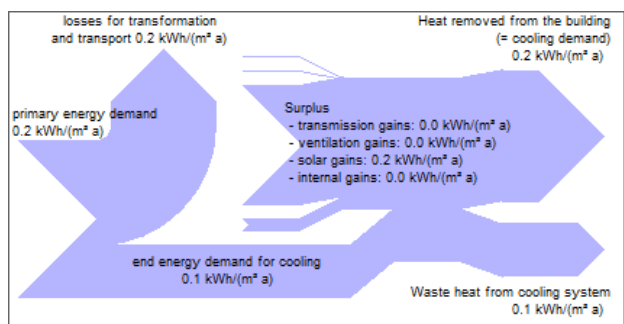
Figure 5. Comparative diagrams of cooling energy required between New Delhi of India (left) and Murmansk of Russia (right)
