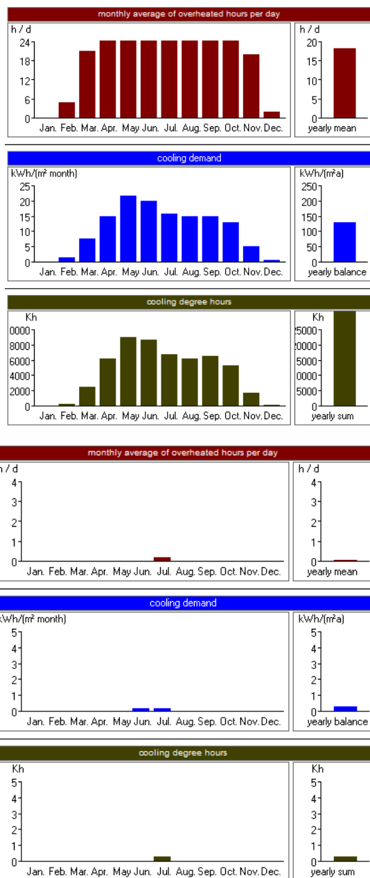
Figure 7. Comparative diagrams of the warm days of the year/ cooling energy requirement/ annual cooling degree in New Delhi (up) and Murmansk of Russia (down)
