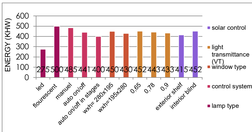
Figure 3. Total annual lighting energy requirements of the alternatives for the office
